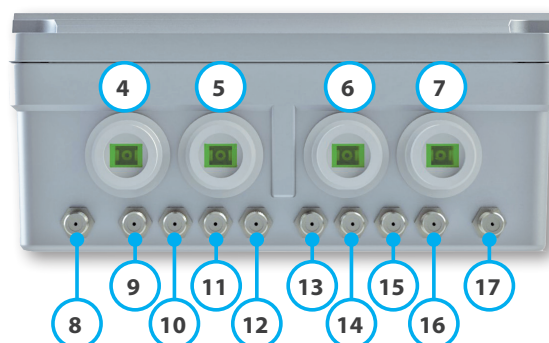
mod. ROF4-RX
