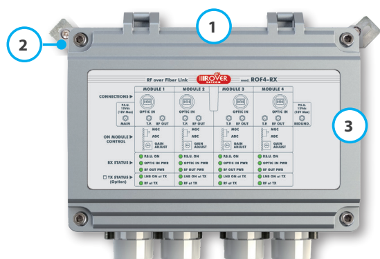
mod. ROF4-RX
