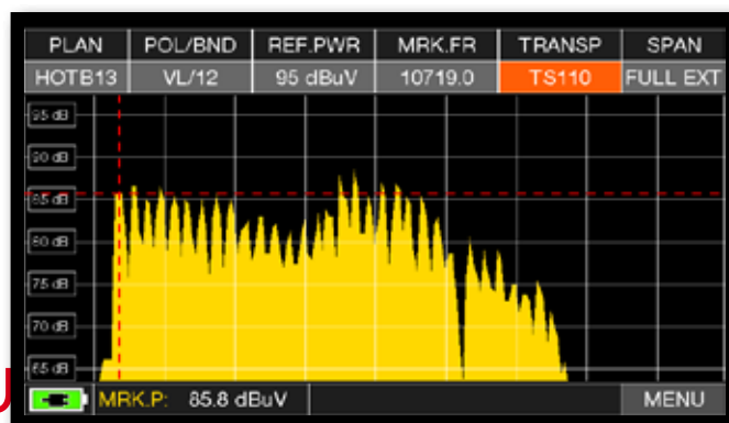
"SAT" spectrum SPAN FULL EXT (from 700 to 2700 MHz) with universal LNB.
