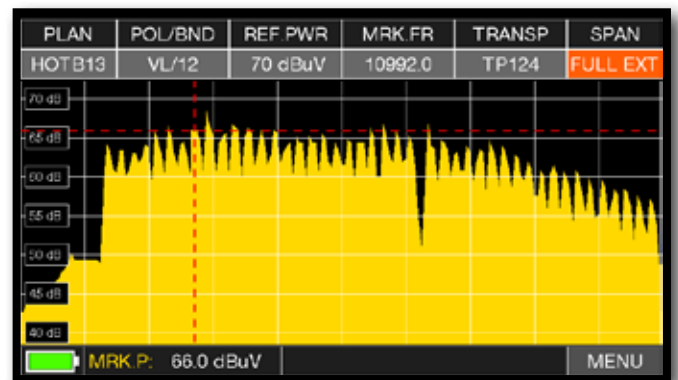
SAT spectrum SPAN "Full EXT" (from 700 to 2700 MHz).
